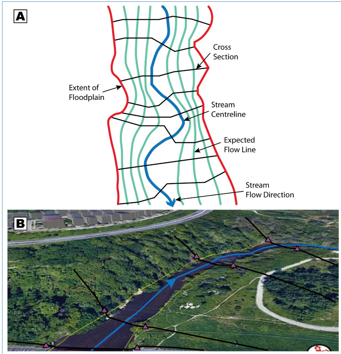
Figure 3-2: Cross sections (cut lines) in hydraulic model showing perpendicular orientation at river centroid as well as: (A) how flow lines are anticipated to look in overbank areas (source: Goodell, 2012); and (B) cross sections with respect to the broader landscape topography and land use, with bank stations shown as purple triangles (image adapted from CivilGEO, 2022). Symbology adapted from federal guidance (NRCan, 2019a).
