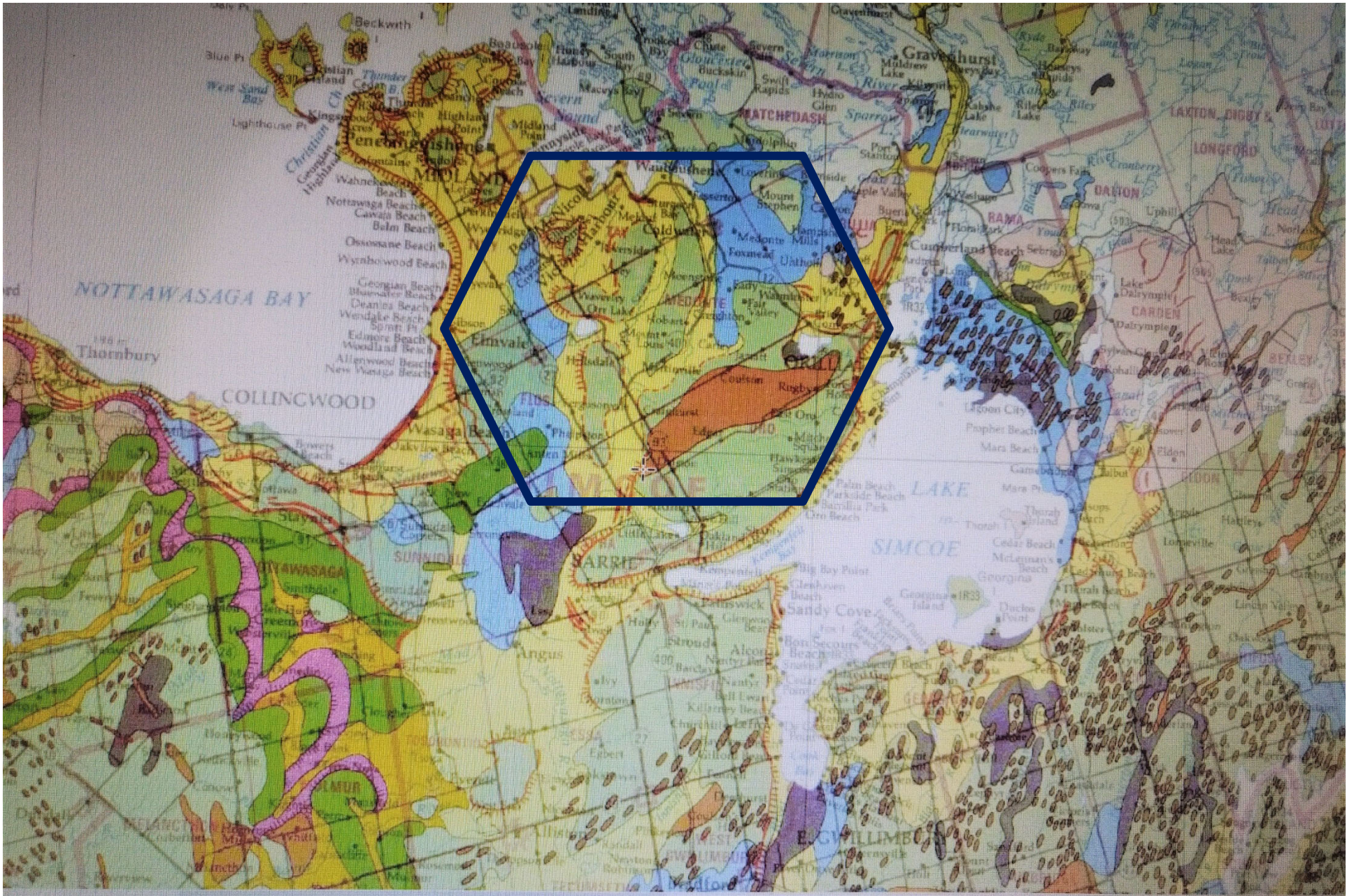
APPROXIMATE location of proposed Bluebelt of groundwater protection
